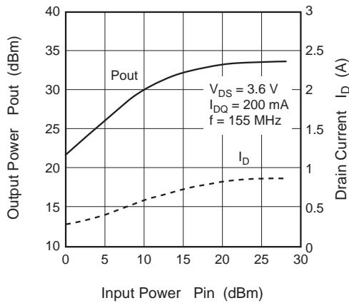
Output Power, Drain Current vs. Input Power
